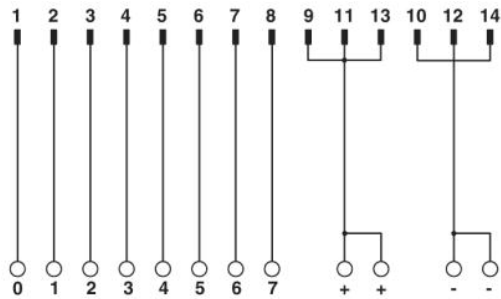
UM 45-FLK14/PLC connection scheme
